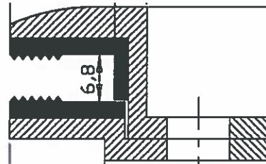
Figure 2: MP-Tec laminate clamp FS4 End Clip
