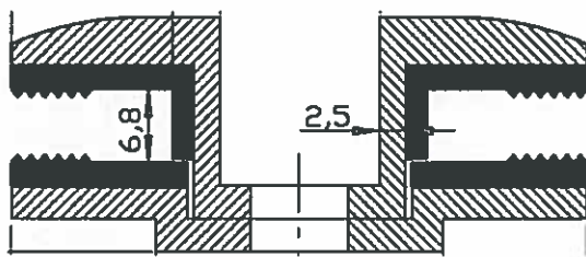
Figure 1: MP-Tec laminate clamp FS4 Mid Clip
